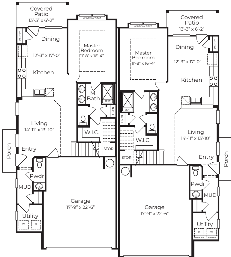
First Floor
